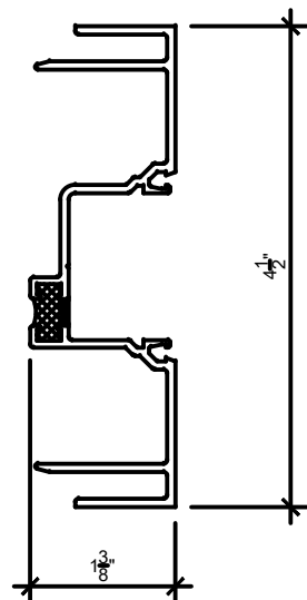
9 FEMALE EXPANSION VERTICAL SCALE: 6" = 1'-0"
