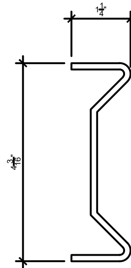
29 STEEL REINFORCEMENT SCALE: 6" = 1'-0"
